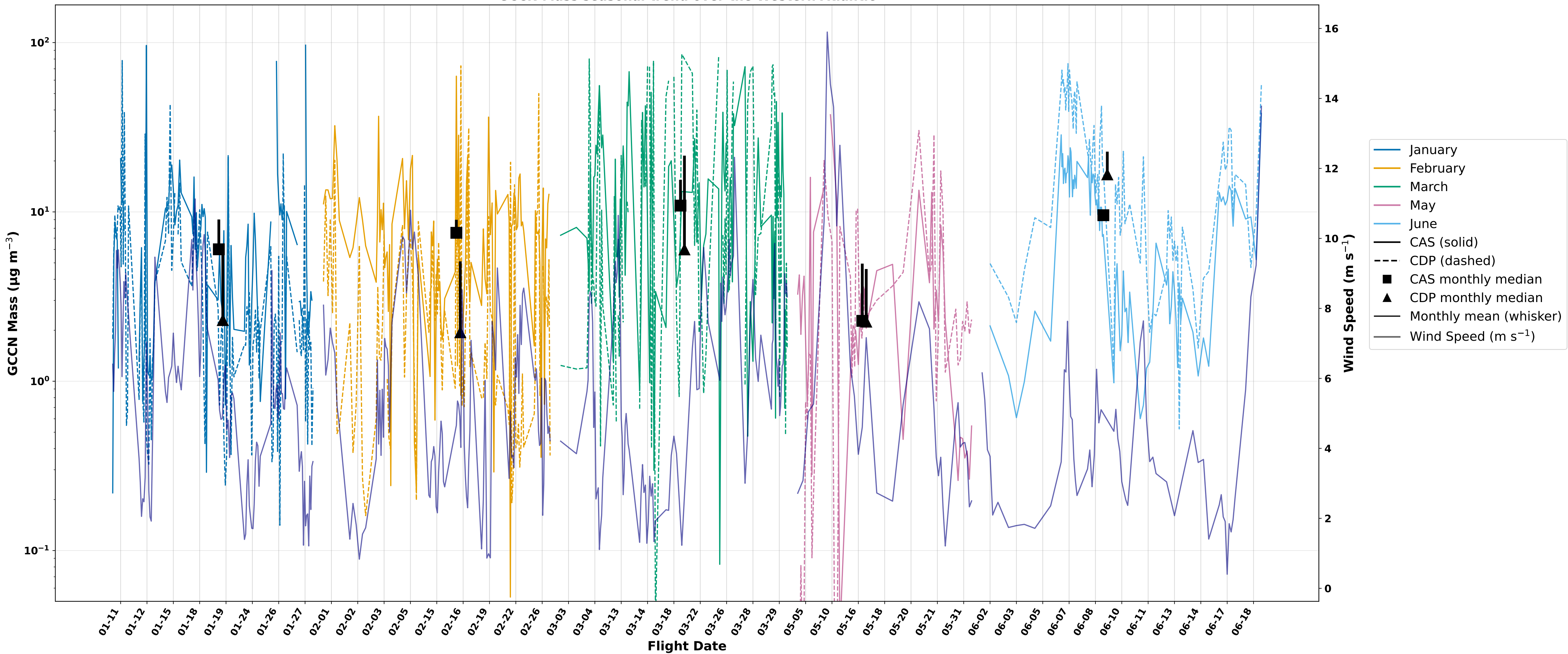
GCCN Mass seasonal trend over the Western Atlantic
